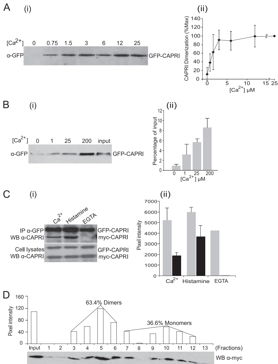
FIGURE 5. Ca^{2+} dependence of CAPRI dimerization. A , CAPRI dimerization requires the presence of Ca^{2+} . GFP-CAPRI was overexpressed in COS-7 cells. The cells were lysed in buffer containing 2 mM Ca^{2+} . Immunoprecipitation was carried out with anti-GFP polyclonal antibody and protein A-Sepharose beads, and the beads were washed in buffers containing the indicated concentrations of Ca^{2+} . Dimerized GFP-CAPRI was eluted with lysis buffer containing 1 mM EGTA and subjected to Western blotting with anti-GFP monoclonal antibody. Panel i , Representative Western blot. Panel ii , quantification by densitometric scanning of Western blots. Data are mean \pm S.D. of three independent experiments. B , Ca^{2+} is sufficient to drive dimerization of purified GFP-CAPRI in vitro . Monomeric GFP-CAPRI was prepared as detailed under "Experimental Procedures," and one-half was kept in solution, and the other was immobilized on beads. Aliquots of immobilized and free GFP-CAPRI were recombined in the presence of the indicated concentrations of Ca^{2+} . Dimerized GFP-CAPRI was eluted with buffer containing 1 mM EGTA and subjected to Western blotting with anti-GFP monoclonal antibody. Panel i , representative Western blot. Input , 5% of the total GFP-CAPRI in each reaction. Panel ii , quantification of dimerized GFP-CAPRI as the percentage of total input. Data are mean \pm range of two independent experiments. C , dimerization of CAPRI can be induced by histamine stimulation of HeLa cells. GFP-CAPRI and myc-CAPRI were co-overexpressed in HeLa cells. The cells were either lysed in buffer containing 1 mM Ca^{2+} or stimulated with 100 \mu M histamine before lysis in Ca^{2+} buffer or lysed in Ca^{2+} -free buffer containing 0.5 mM EGTA, as indicated. Immunoprecipitation was carried out with anti-GFP monoclonal antibody, and the blots were probed with anti-CAPRI antibody. Panel i , representative Western blot (WB). Panel ii , quantification by densitometric scanning. Data are mean \pm range of two independent experiments, except for EGTA, which are from one experiment. D , quantification of CAPRI monomers and dimers by gel filtration. myc-CAPRI was overexpressed in Cos-7 cells, and the cells were lysed in buffer with 500 \mu M Ca^{2+} . The lysates were subjected to FPLC Superose 12 gel filtration column as detailed under "Experimental Procedures." Column fraction aliquots (30 \mu l /fraction) were subjected to SDS-PAGE and Western blotting with anti-Myc monoclonal antibody. Quantification of the monomeric and dimeric forms of CAPRI was obtained by densitometric scanning. One-tenth input proteins were loaded in the input lane. The standard protein markers are blue dextran 2000 kDa, apoferritin 443 kDa, \beta -amylase 200 kDa, alcohol dehydrogenase 150 kDa, BSA 66.2 kDa, carbonic anhydrase 29 kDa, cytochrome c 12.4 kDa, and aprotinin 6500 Da.
