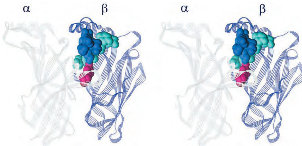
FIG. 5. Stereoscopic representation of the \beta 2 residues conferring up-regulation to \alpha 3\beta 4 receptor. The model of the extracellular domain of \alpha 3\beta 2 is based on the crystal structure of AChBP (34). Residues belonging to the \beta 2 segment (74–89) are shown in blue and belonging to the \beta 2 segment (106–115) are in cyan. These residues form a compact microdomain located at the interface between \alpha (light gray) and \beta 2 (dark blue) and contact the upper part of the nicotinic site. Epibatidine is shown in pink, according to previous docking calculations (30).
